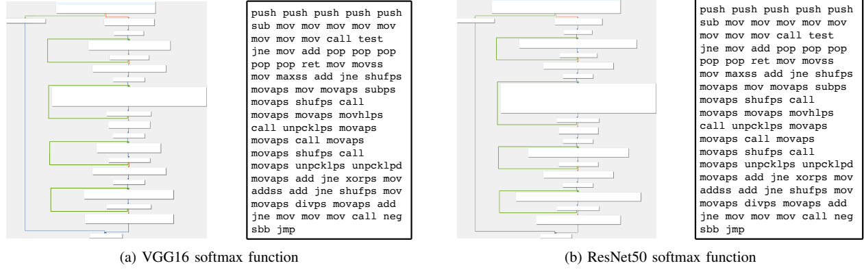
Fig. 2: Comparison of CFG and Opcode sequence of softmax function between VGG16 (Fig.2a) and ResNet50 (Fig.2b) DNN Programs, compiled by TVM with optimization -O0.
